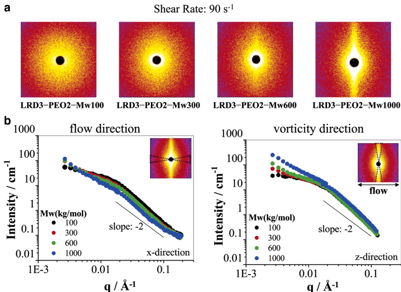
Figure 8. (a) 2D SANS profiles of samples at a shear rate of 90 \text{ s}^{-1} . Anisotropic SANS patterns observed at the samples with M_w = 300, 600 , and 1000 . (b) Averaged intensity vs q for the samples with different molecular weight, at a shear rate of 90 \text{ s}^{-1} . Left: intensity average parallel to the flow (x-direction). Right: intensity average perpendicular to the flow (z-direction). Inserts: 2D SANS anisotropic scattering patterns showing the sectors used for averaging the intensity.
